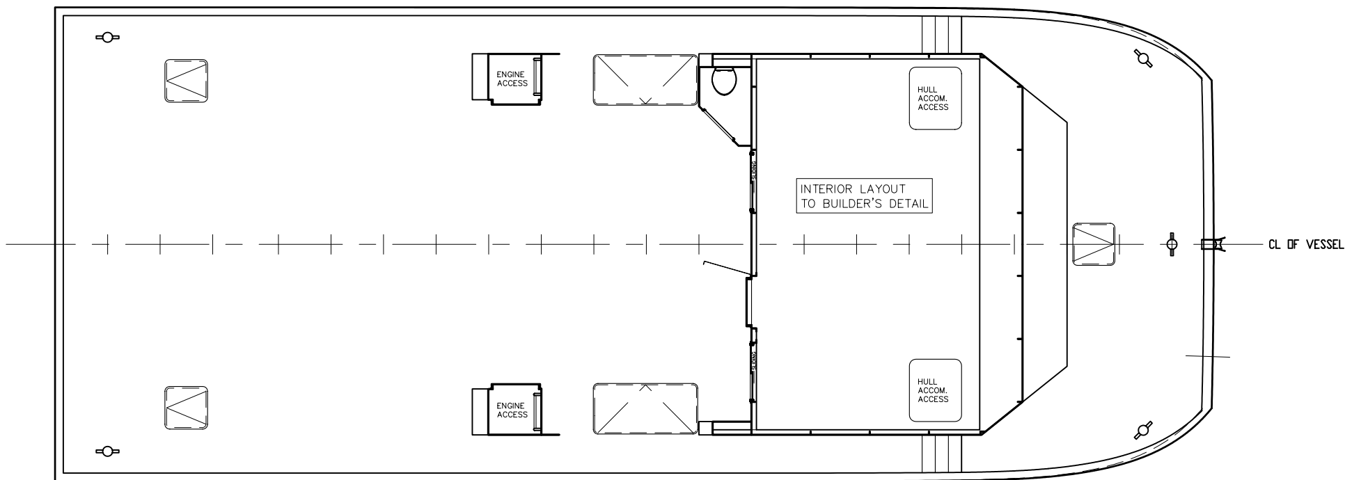
MAIN DECK PLAN
