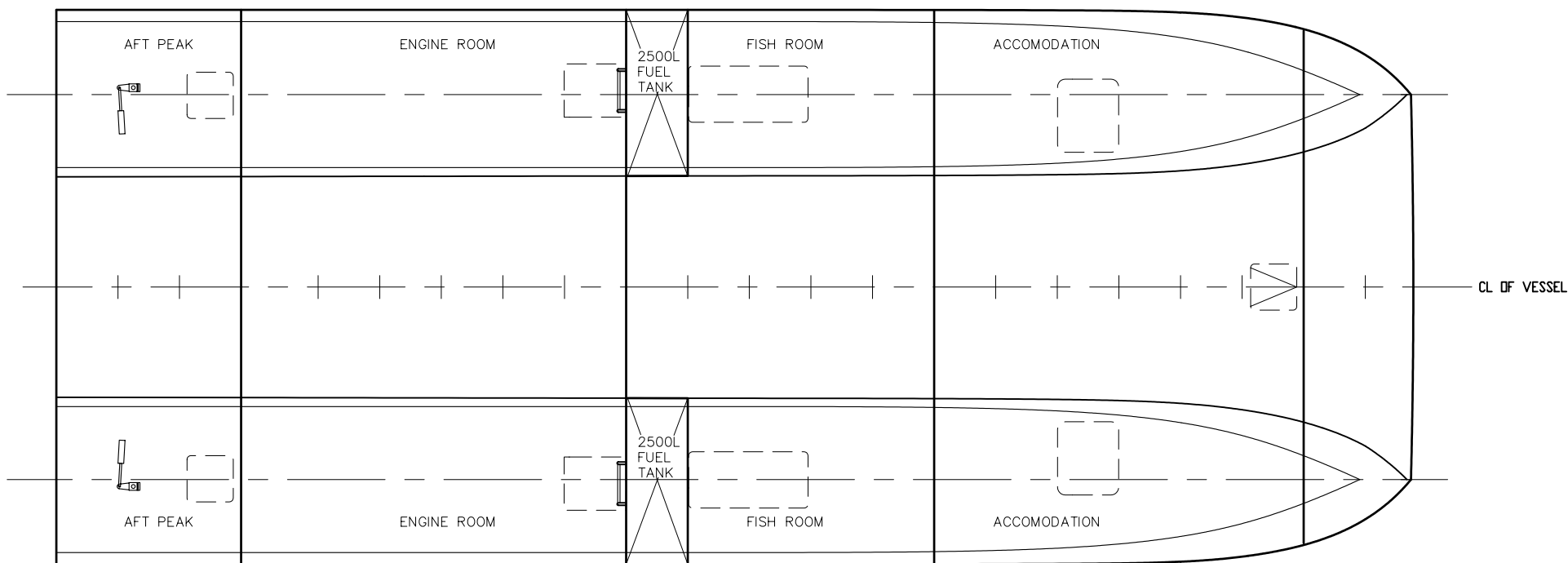
UNDER DECK PLAN
